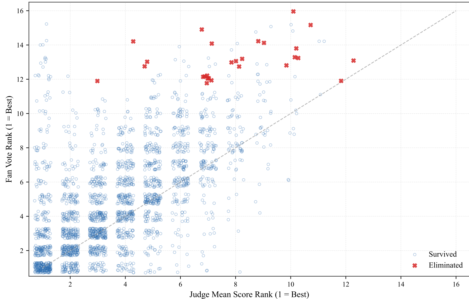
Fan Rank vs. Judge Mean Rank
