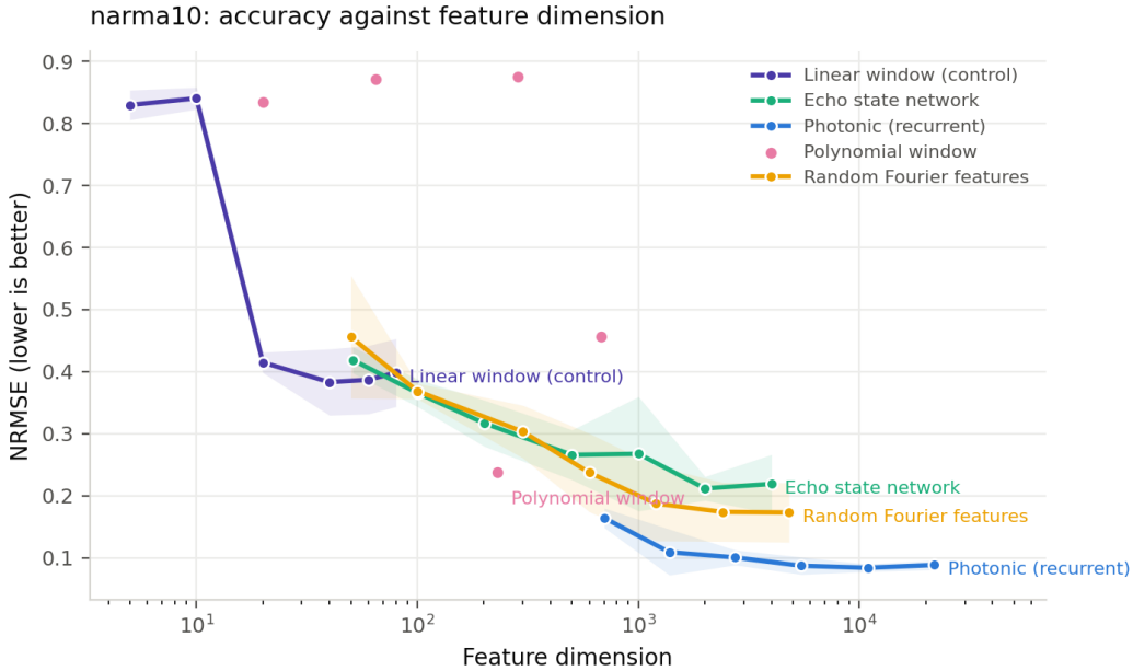
Figure 1: NRMSE against feature dimension on NARMA-10. The echo state network saturates beyond \sim 2000 units; the photonic map does not. A single photonic reservoir at 701 features already matches the echo state network’s best.
