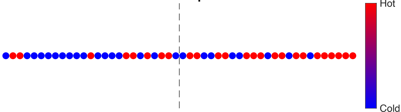
Distribution of particles
