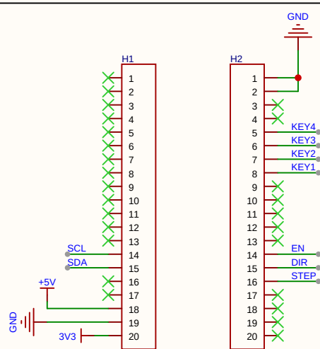
STM32F103C8T6排母
