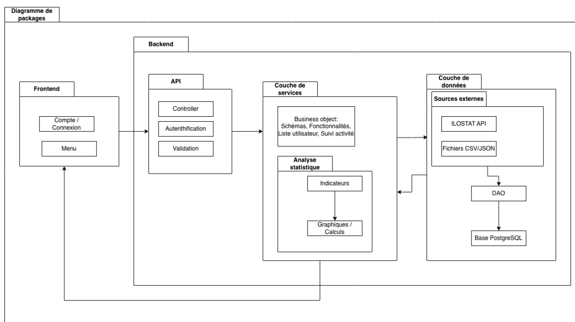
Figure 5. – Diagramme de packages
