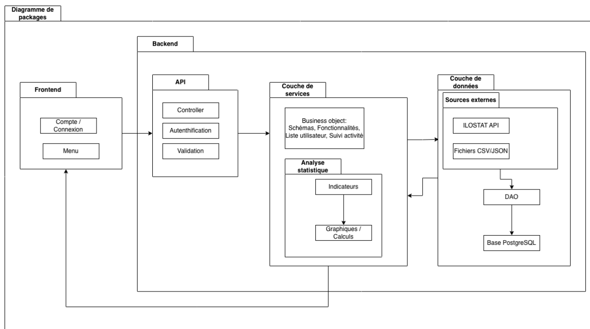
Figure 5. – Diagramme de packages
