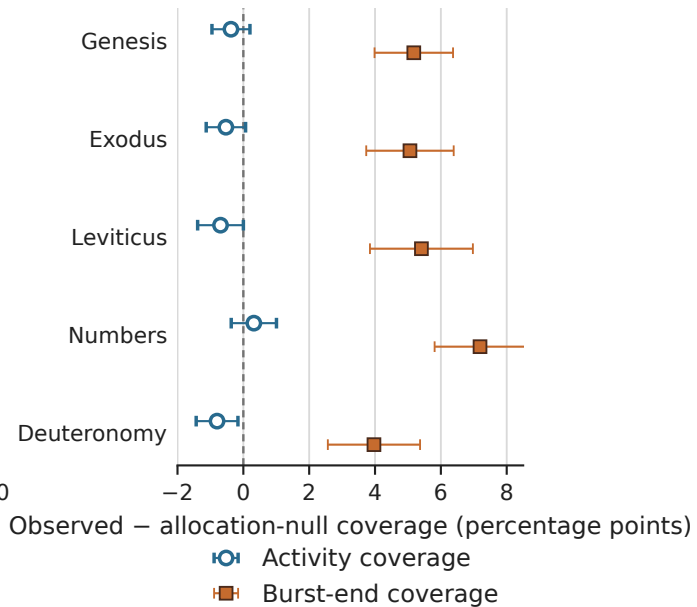
B. Coverage beyond allocation null
