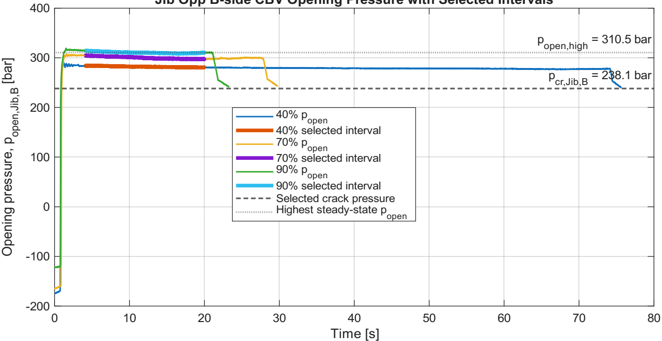
Jib Opp B-side CBV Opening Pressure with Selected Intervals
