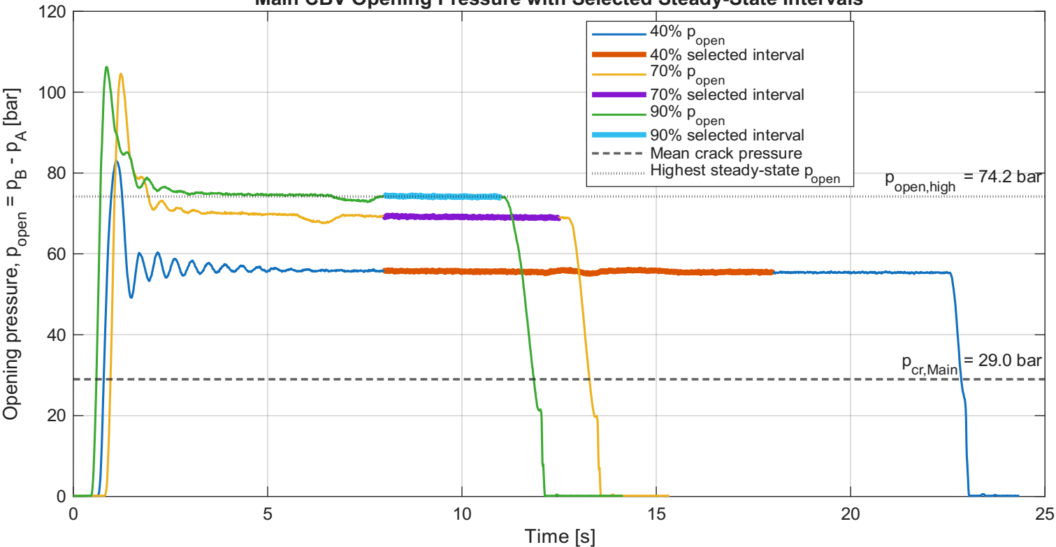
Main CBV Opening Pressure with Selected Steady-State Intervals
