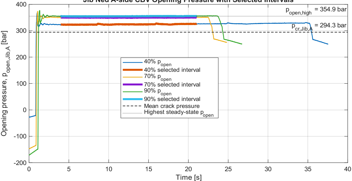
Jib Ned A-side CBV Opening Pressure with Selected Intervals
