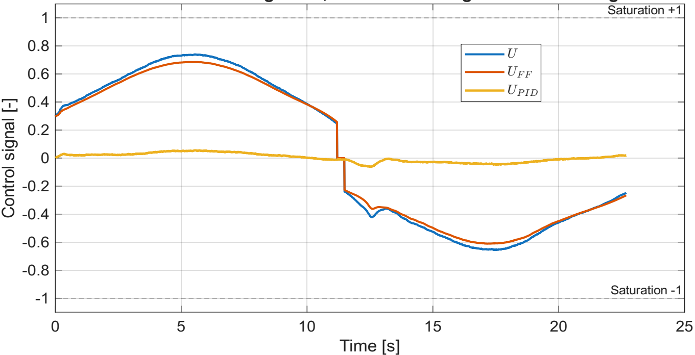
Test 11 - Dual-axis high flow, new flow-sharing - Main control signal
