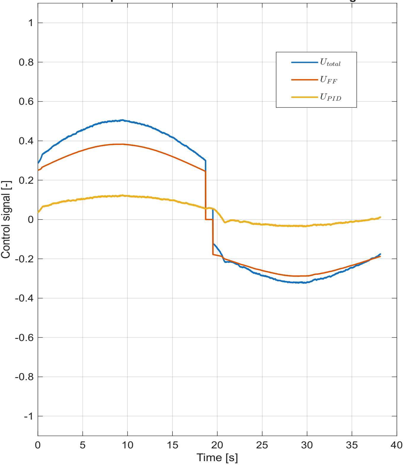
Jib hard position - classical feedforward - control signal
