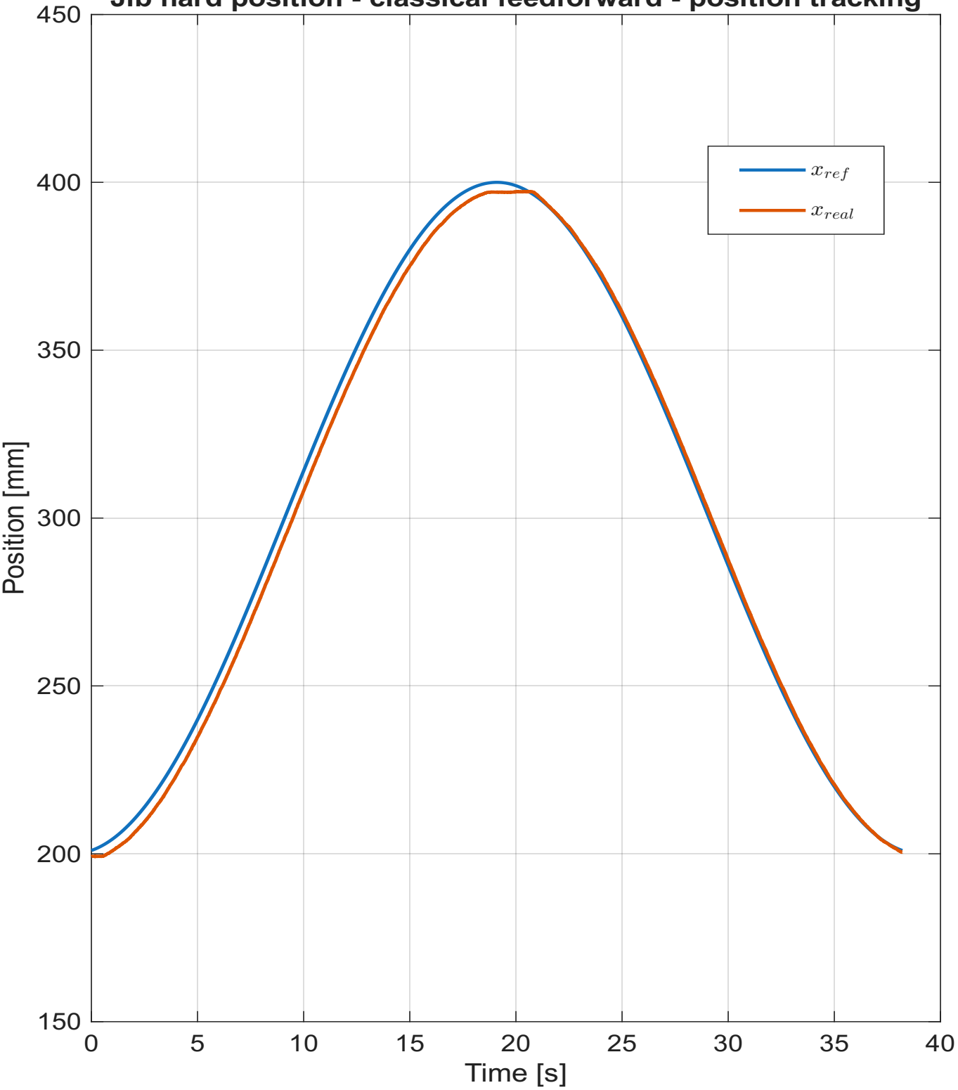
Jib hard position - classical feedforward - position tracking
