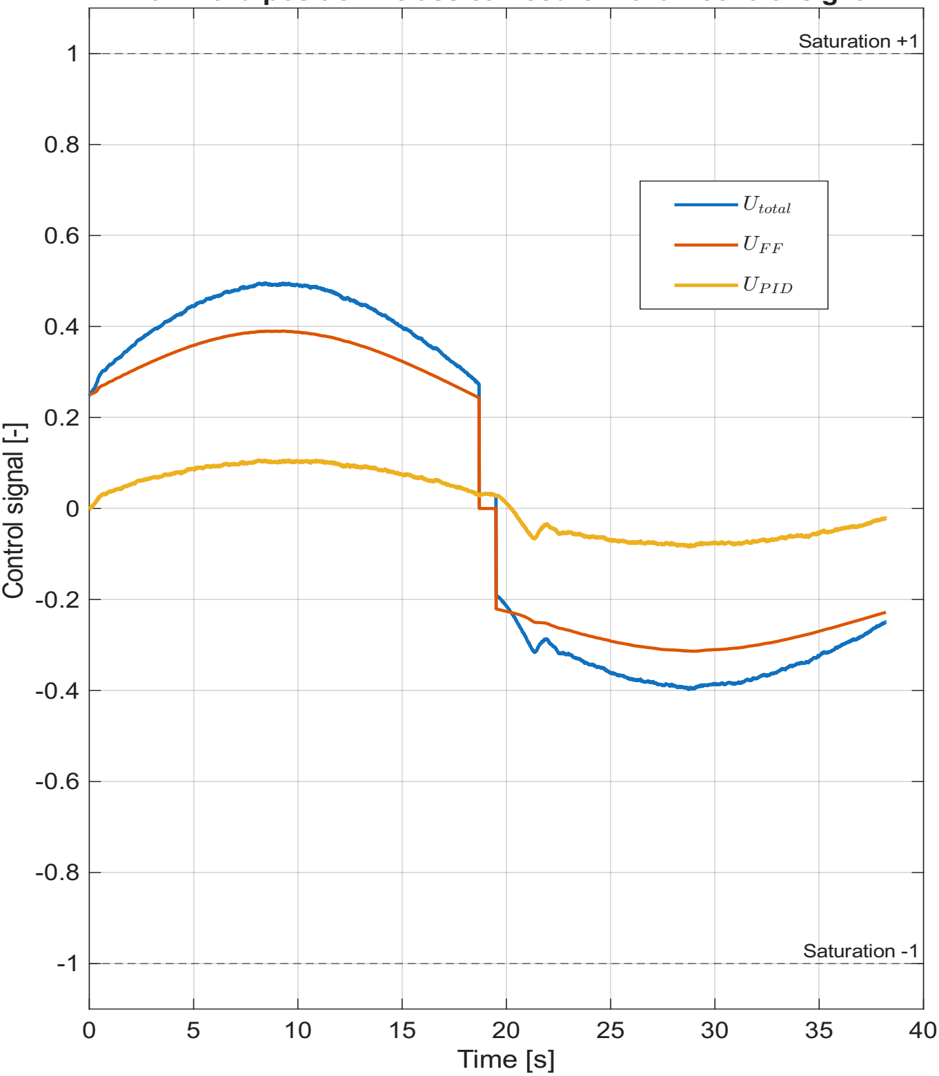
Main hard position - classical feedforward - control signal
