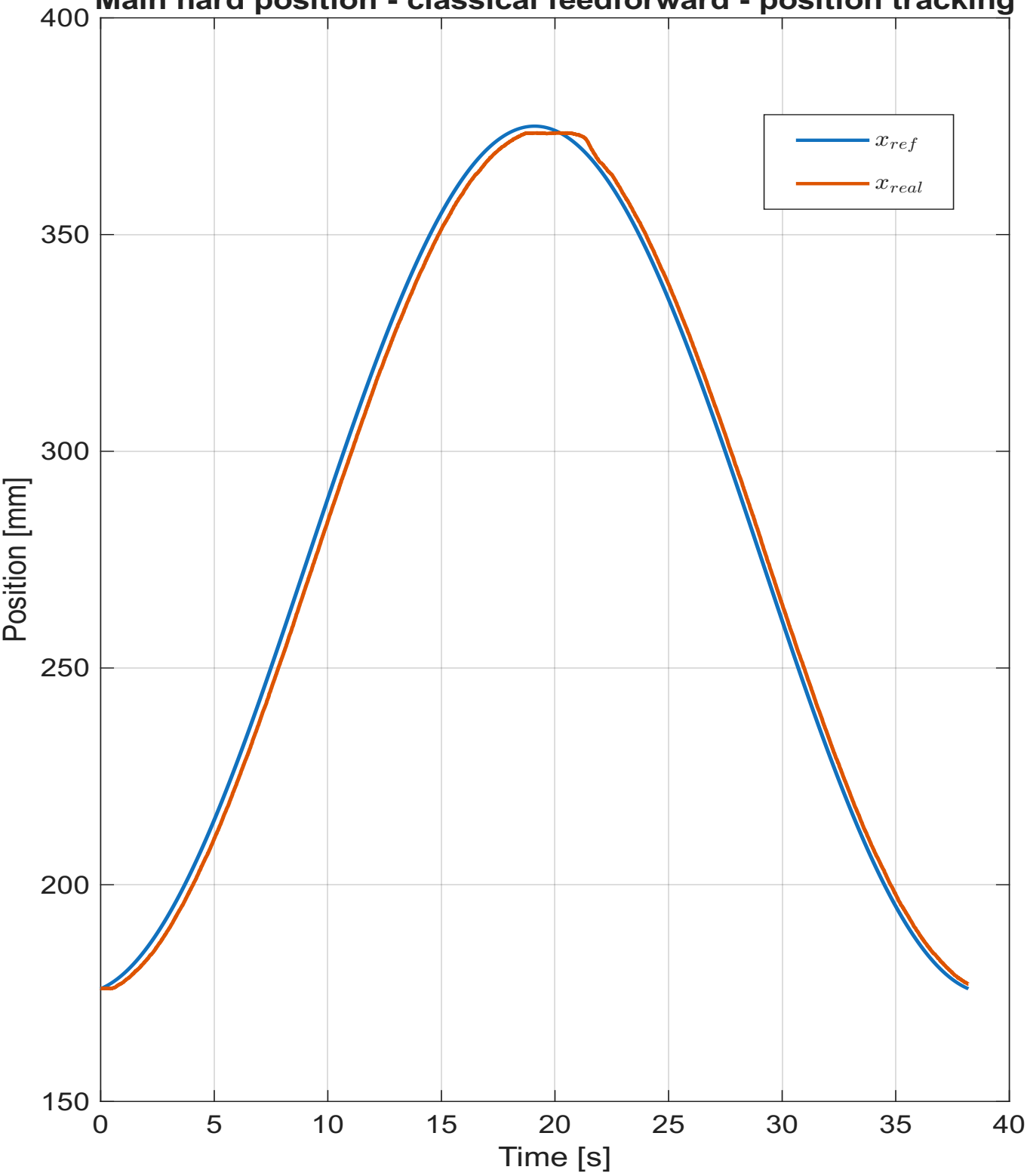
Main hard position - classical feedforward - position tracking
