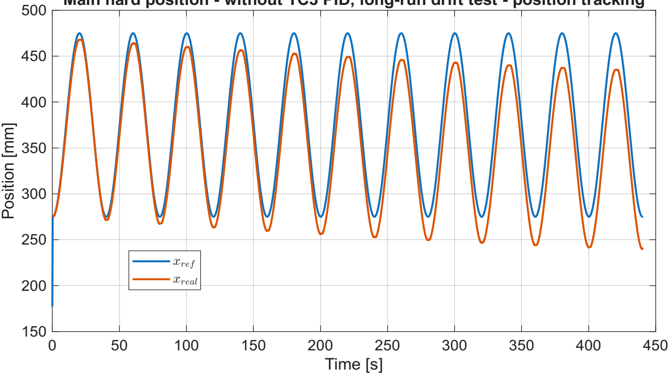
Main hard position - without TC3 PID, long-run drift test - position tracking
