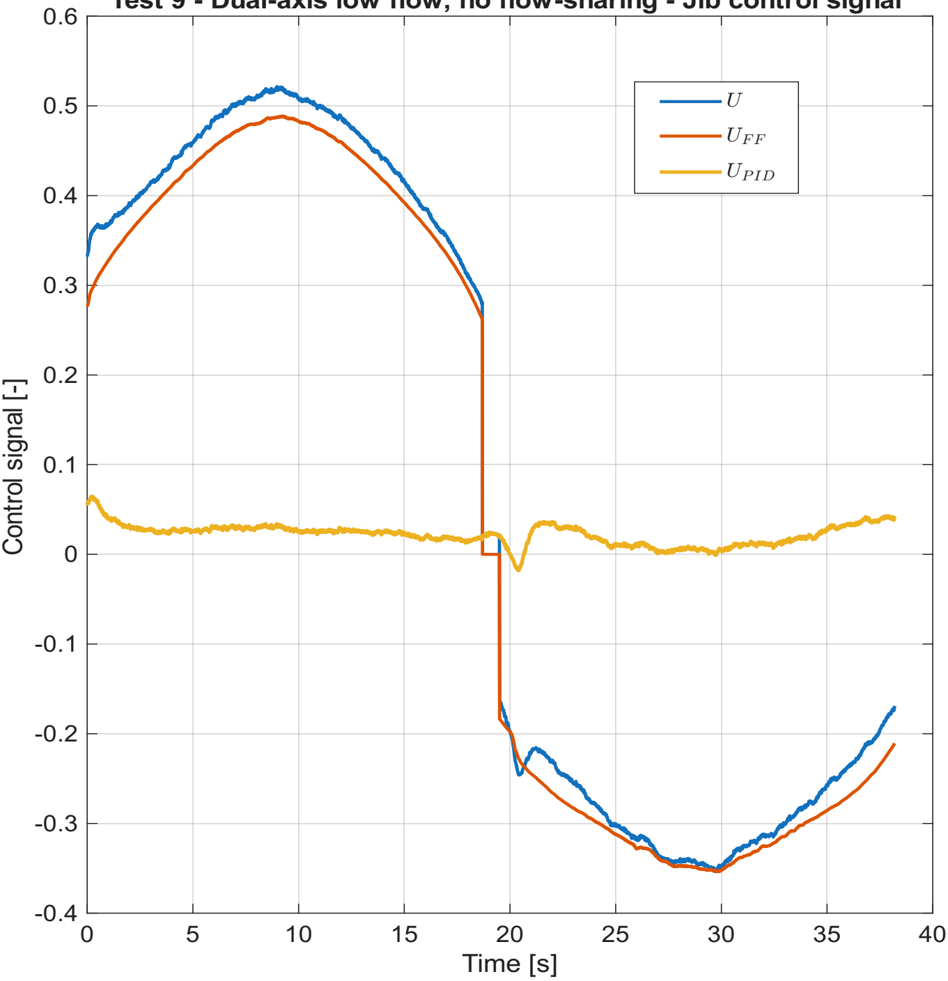
Test 9 - Dual-axis low flow, no flow-sharing - Jib control signal
