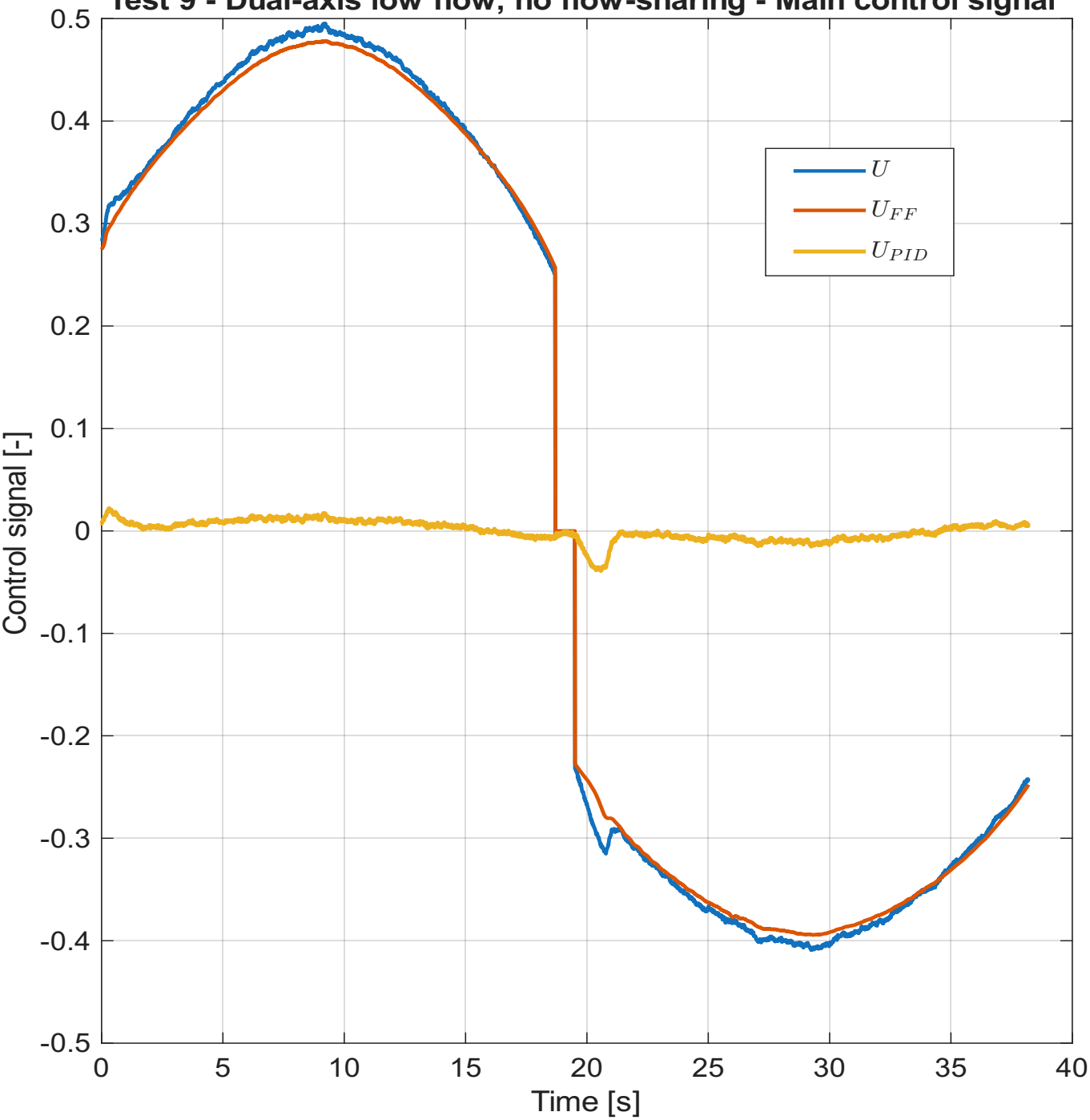
Test 9 - Dual-axis low flow, no flow-sharing - Main control signal
