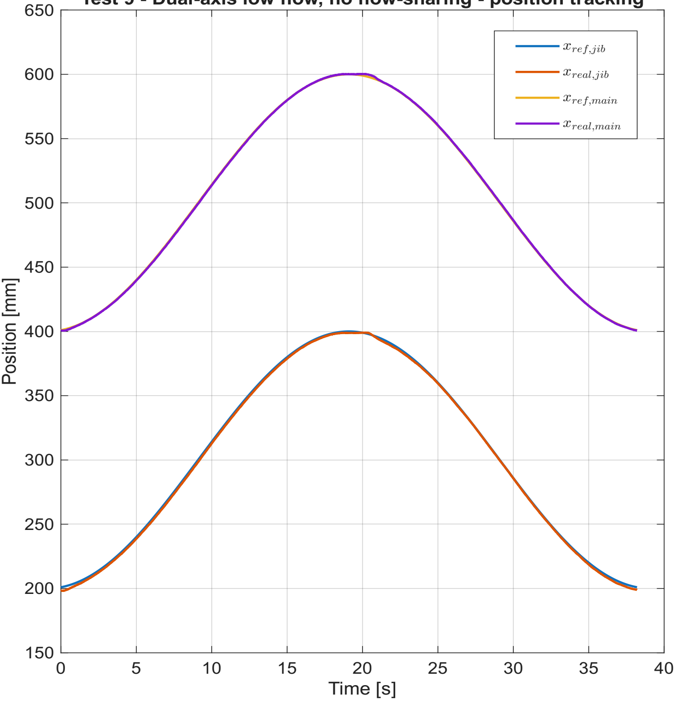
Test 9 - Dual-axis low flow, no flow-sharing - position tracking
