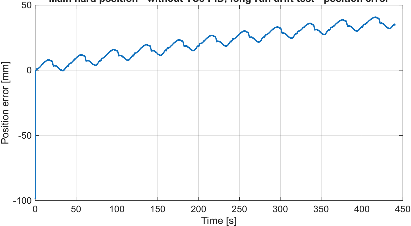
Main hard position - without TC3 PID, long-run drift test - position error
