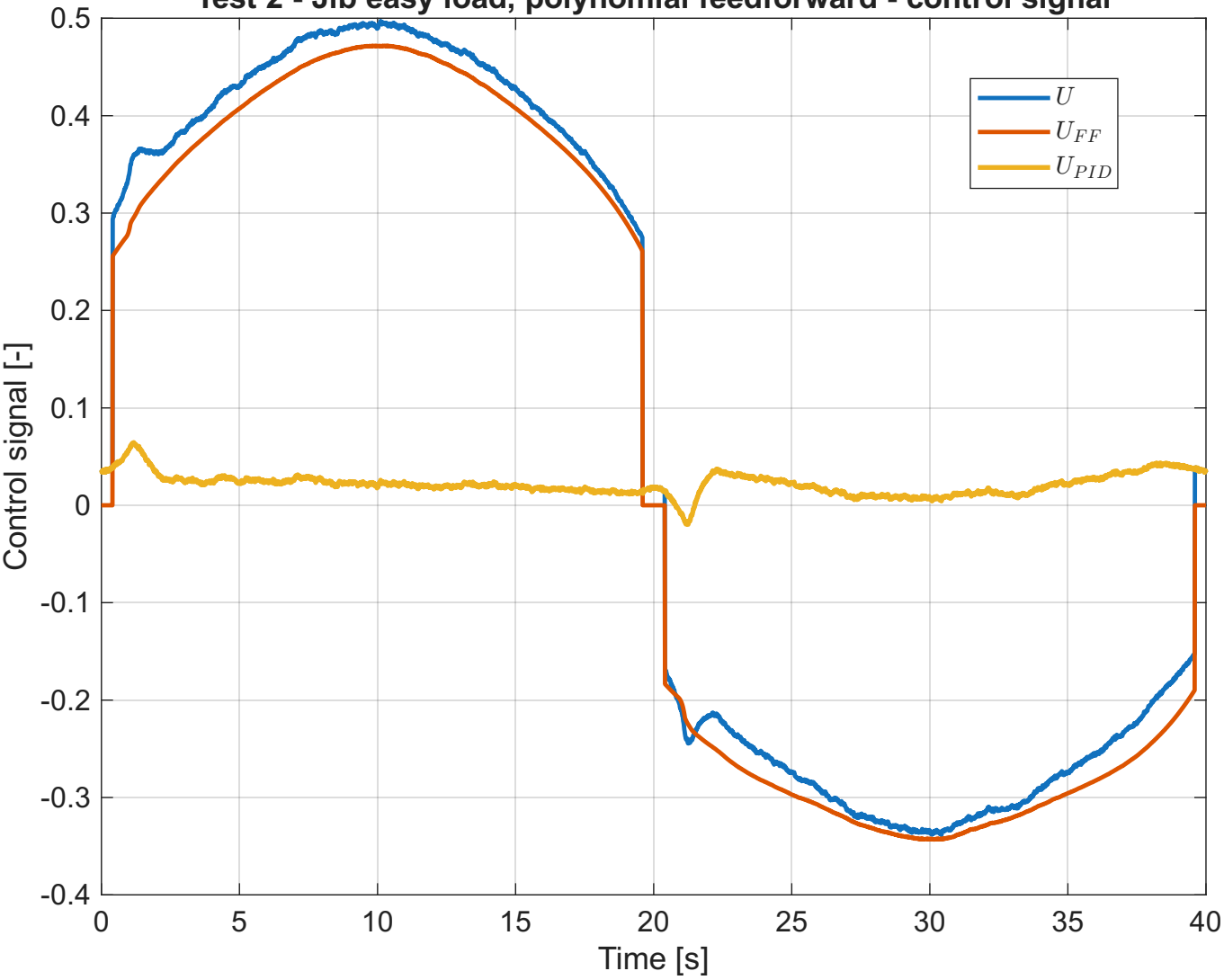
Test 2 - Jib easy load, polynomial feedforward - control signal
