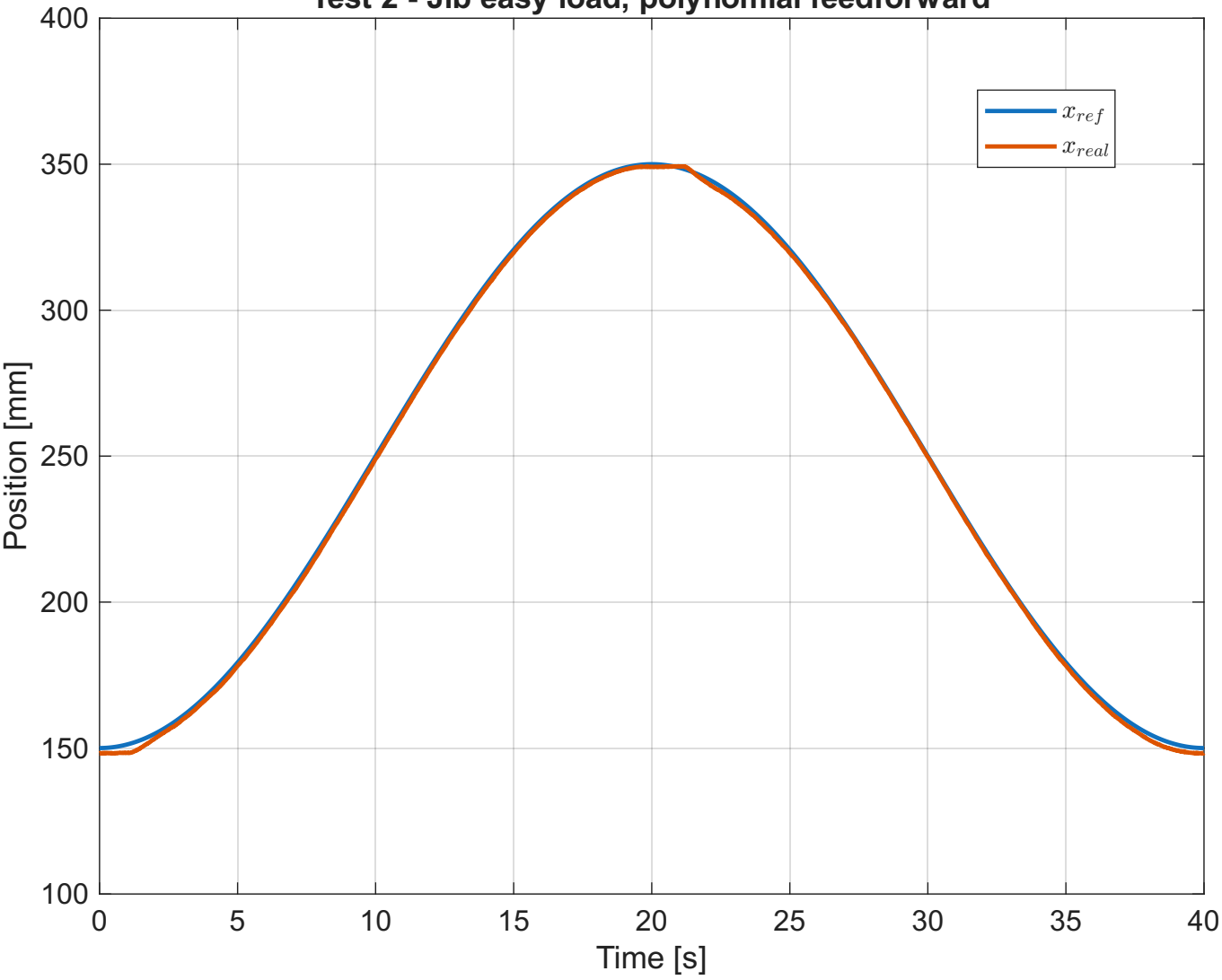
Test 2 - Jib easy load, polynomial feedforward
