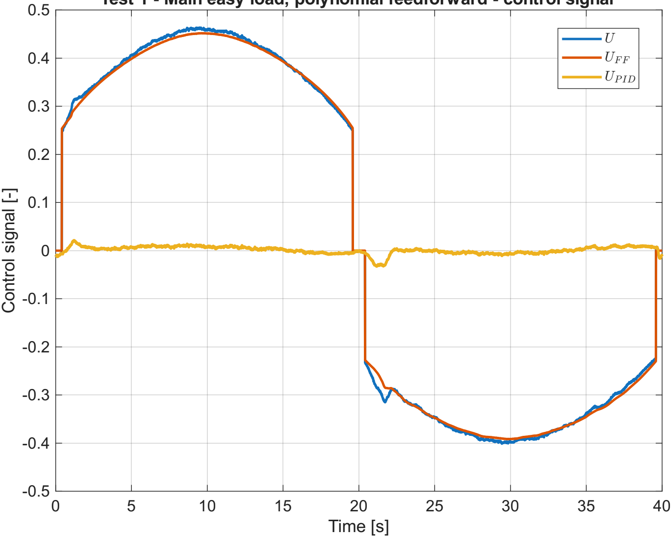
Test 1 - Main easy load, polynomial feedforward - control signal
