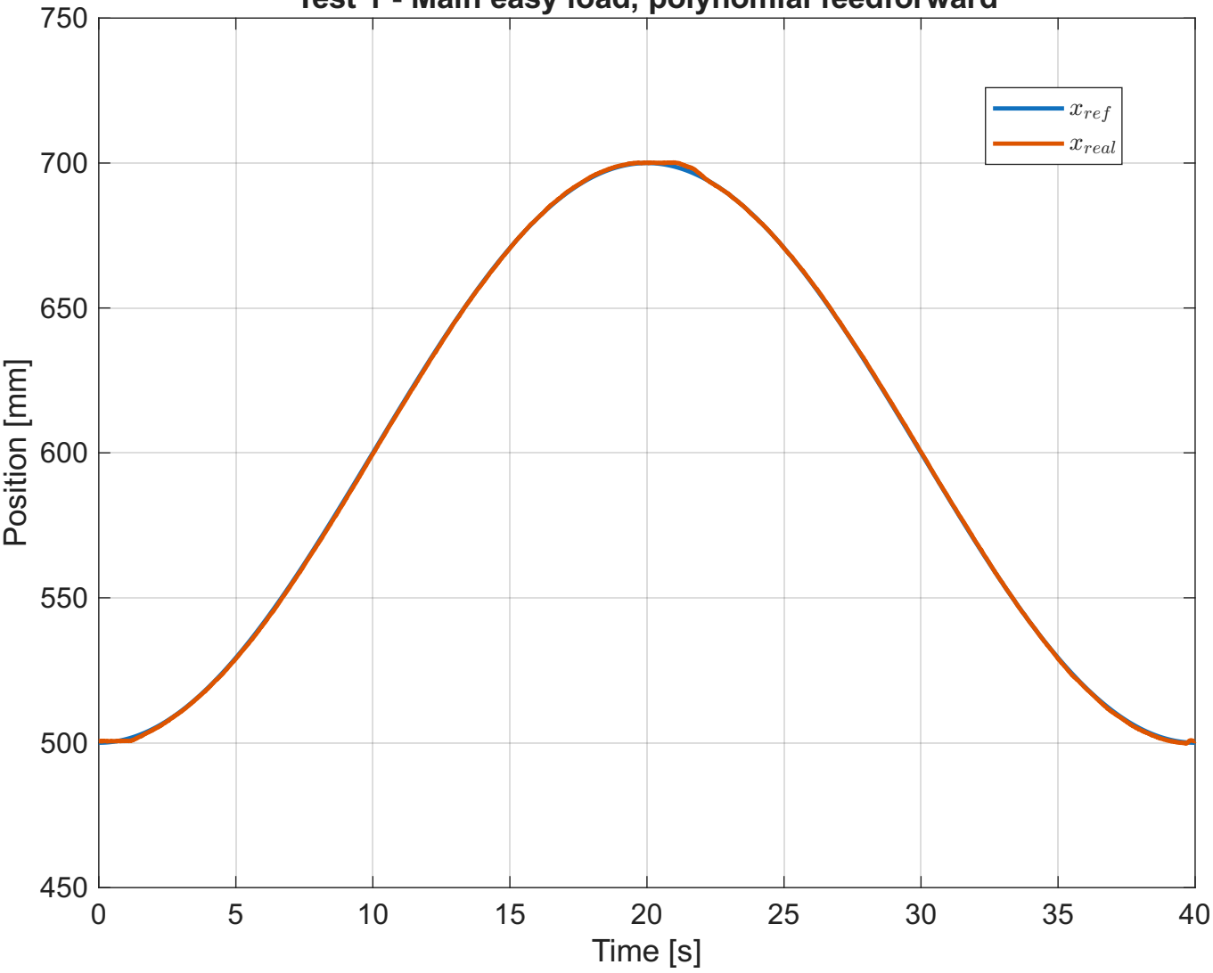
Test 1 - Main easy load, polynomial feedforward
