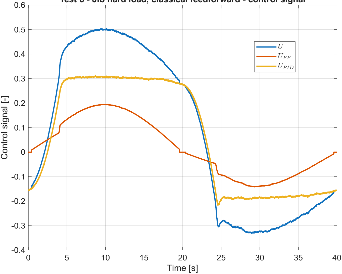
Test 6 - Jib hard load, classical feedforward - control signal
