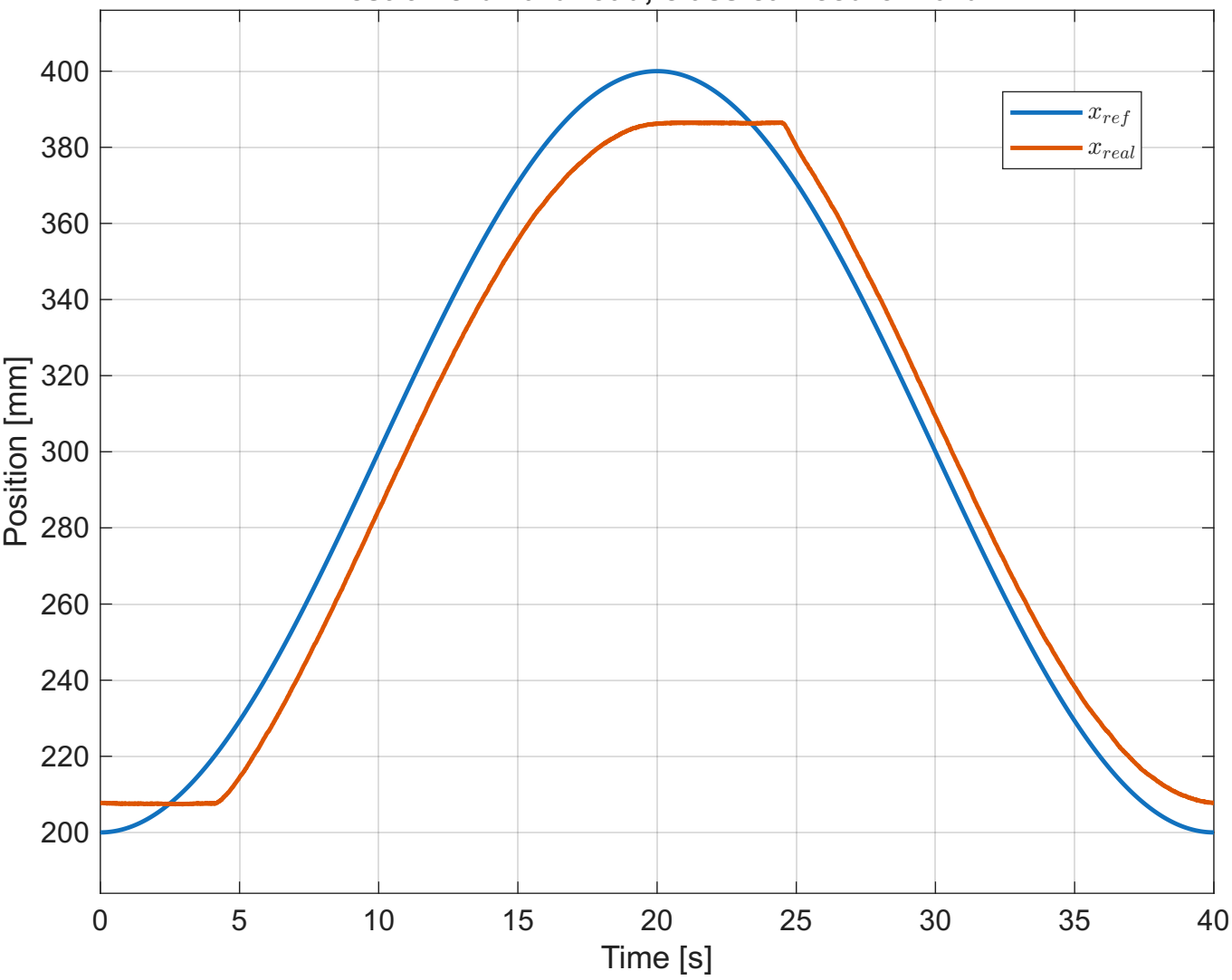
Test 6 - Jib hard load, classical feedforward
