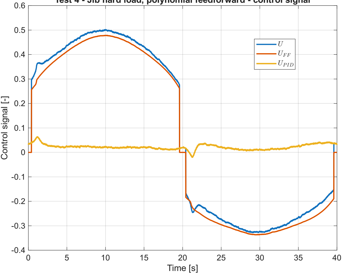
Test 4 - Jib hard load, polynomial feedforward - control signal
