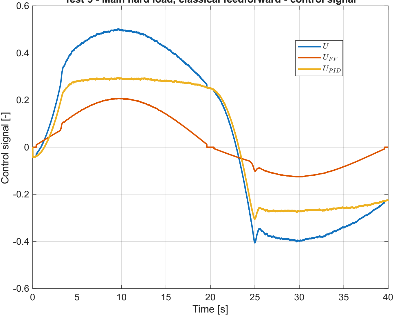
Test 5 - Main hard load, classical feedforward - control signal
