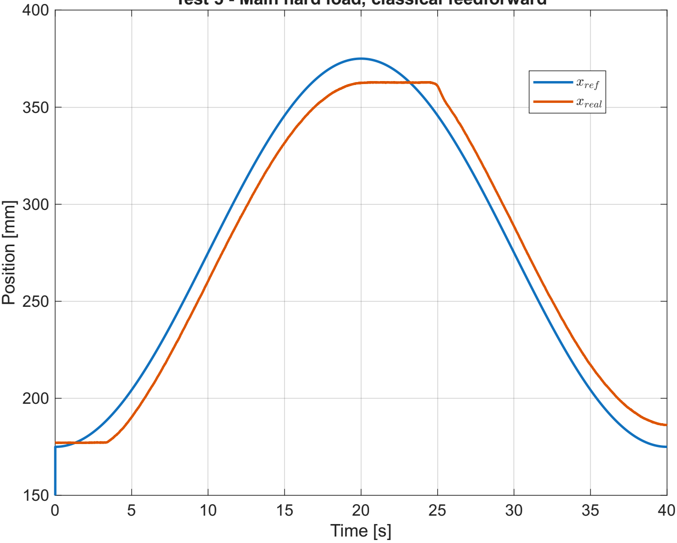
Test 5 - Main hard load, classical feedforward
