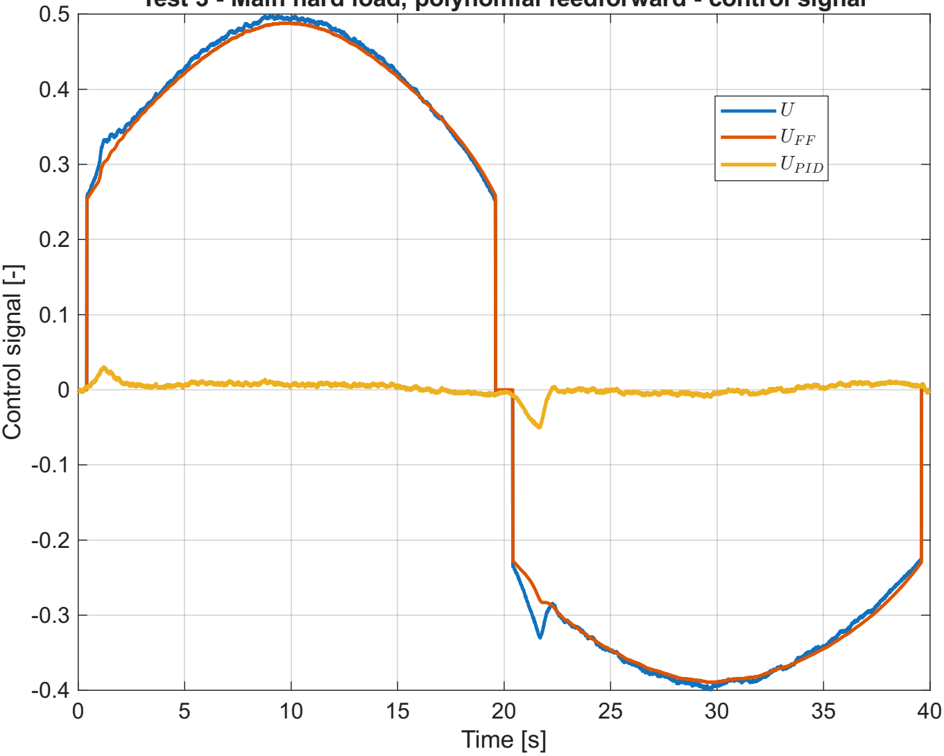
Test 3 - Main hard load, polynomial feedforward - control signal
