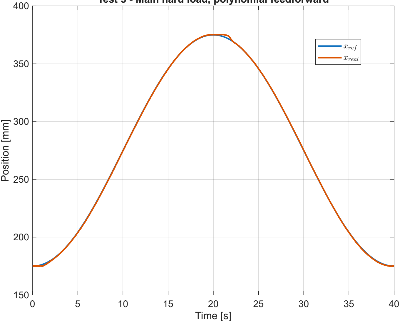
Test 3 - Main hard load, polynomial feedforward
