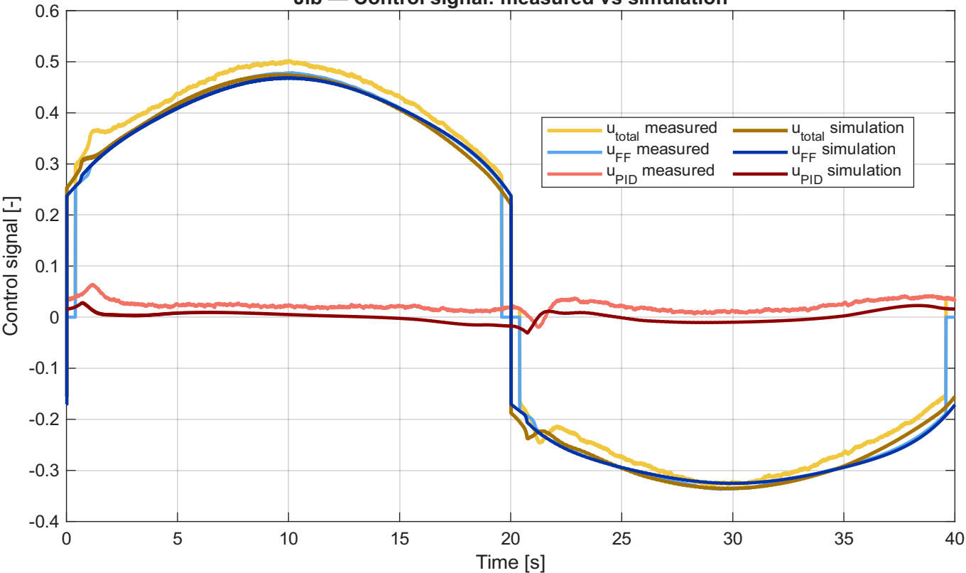
Jib — Control signal: measured vs simulation
