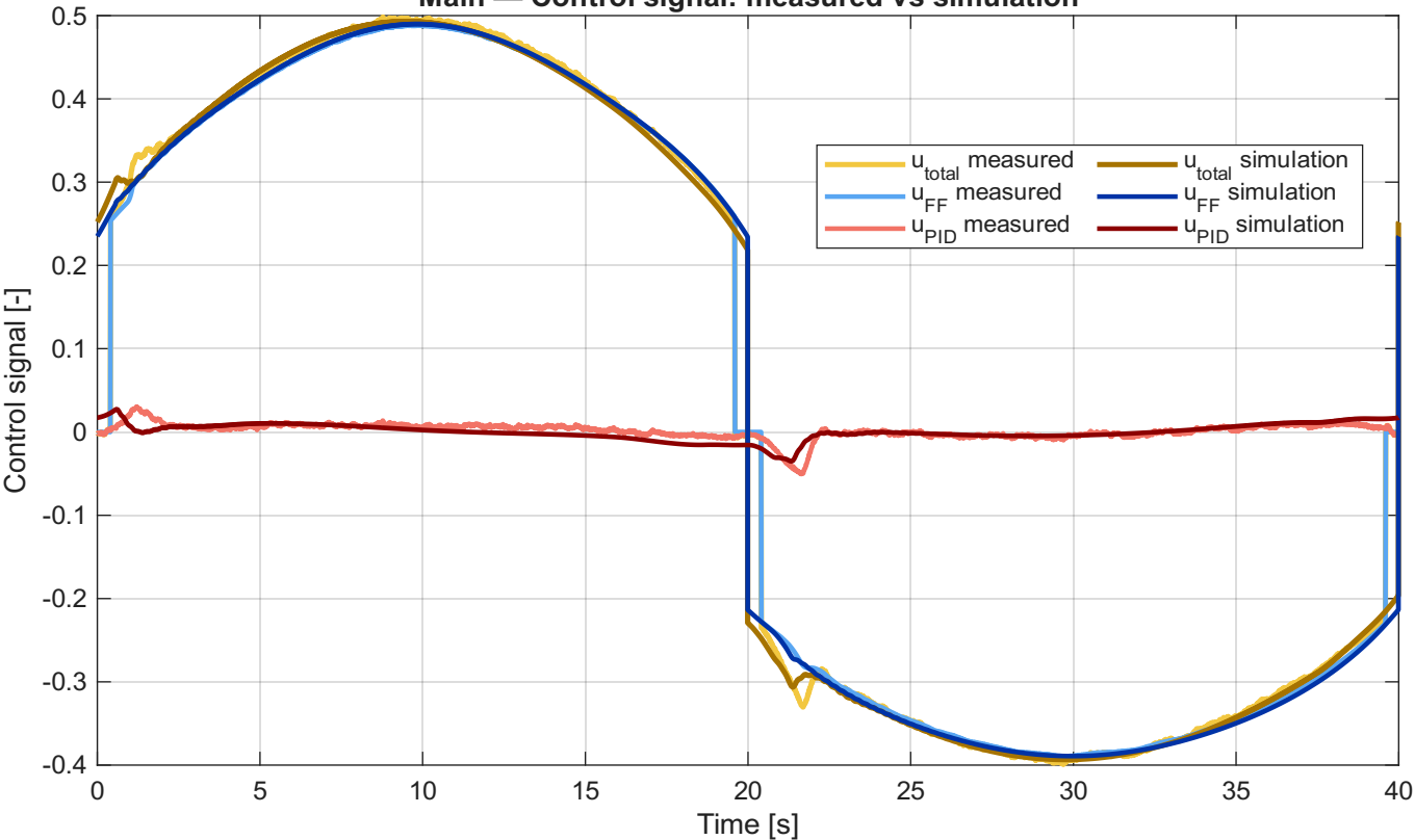
Main — Control signal: measured vs simulation
