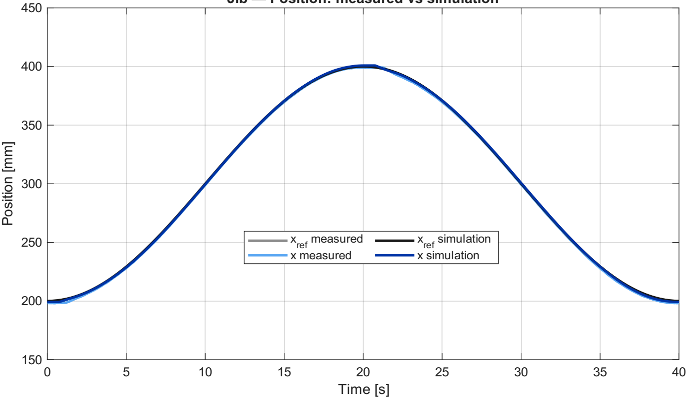
Jib — Position: measured vs simulation
