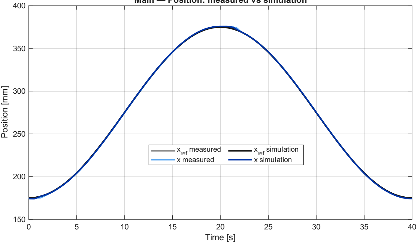
Main — Position: measured vs simulation
