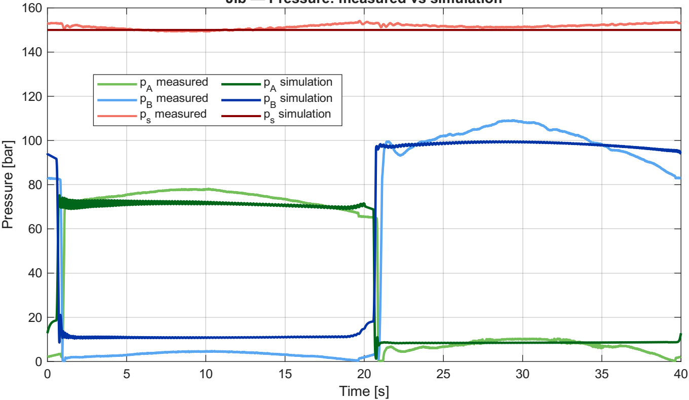
Jib — Pressure: measured vs simulation
