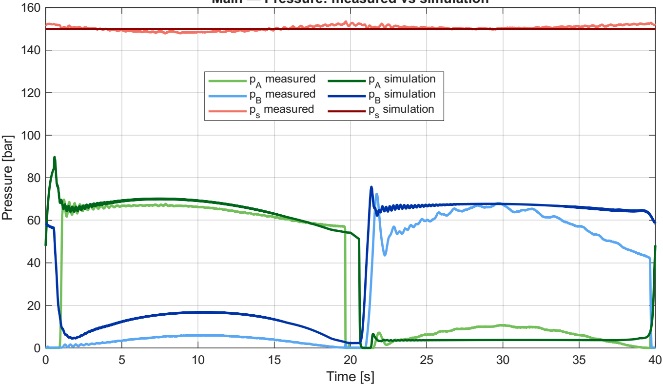
Main — Pressure: measured vs simulation
