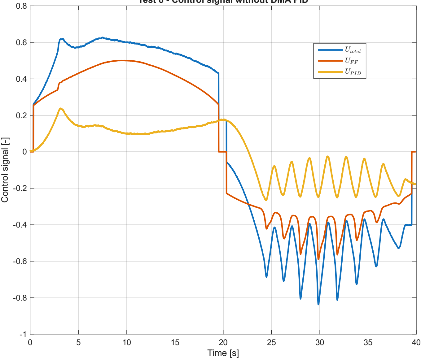
Test 8 - Control signal without DMA PID
