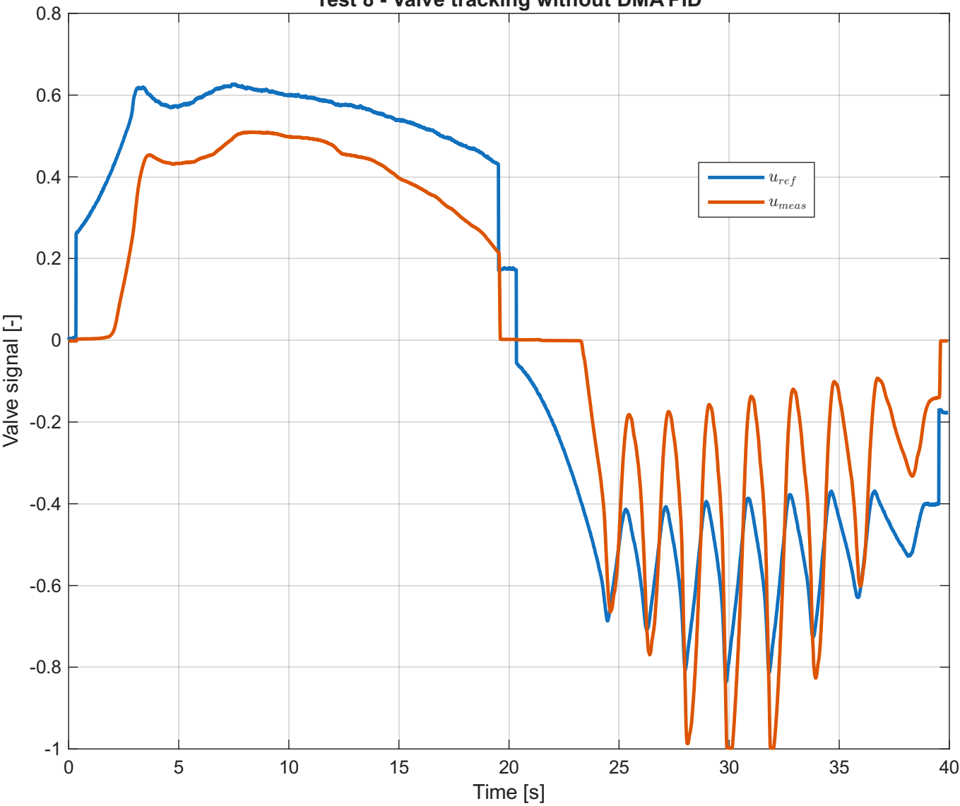
Test 8 - Valve tracking without DMA PID
