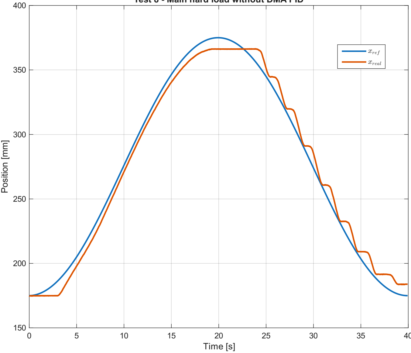
Test 8 - Main hard load without DMA PID
