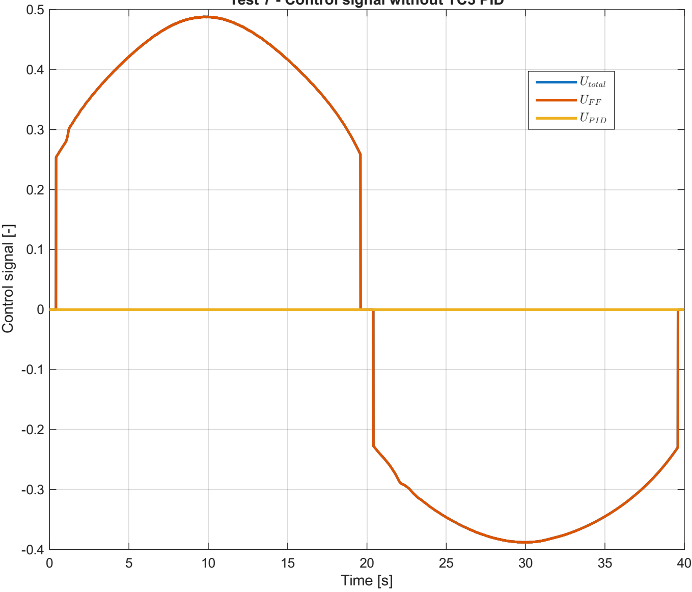
Test 7 - Control signal without TC3 PID
