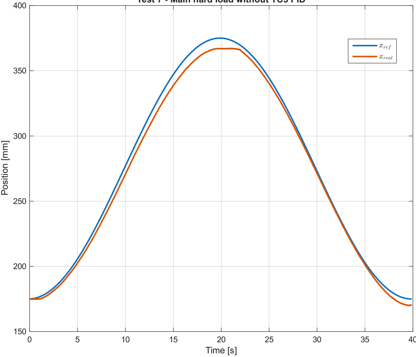
Test 7 - Main hard load without TC3 PID
