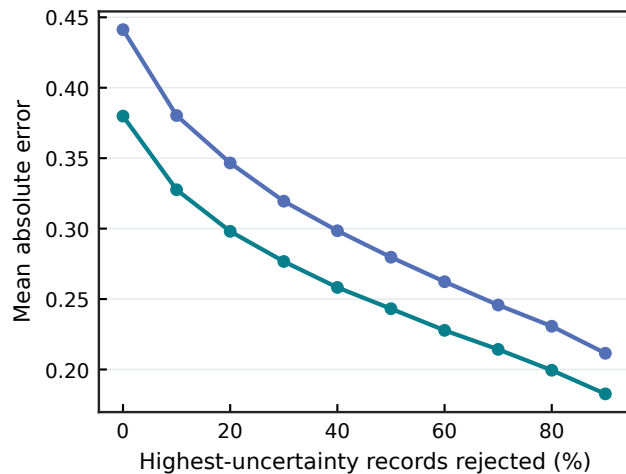
D Error after uncertainty rejection
