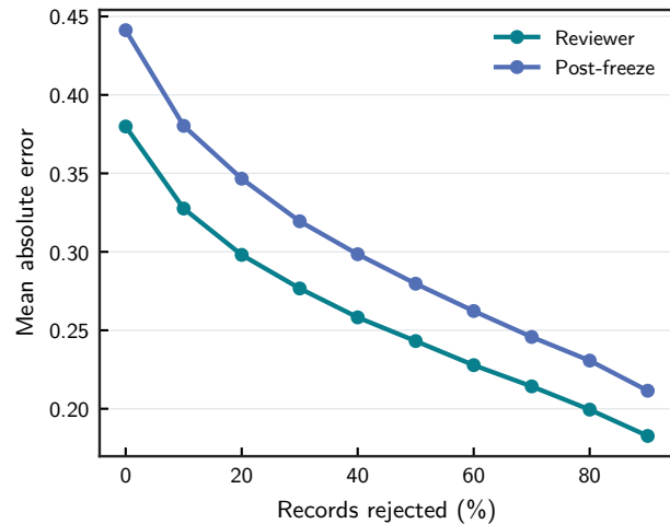
D Error after uncertainty rejection
