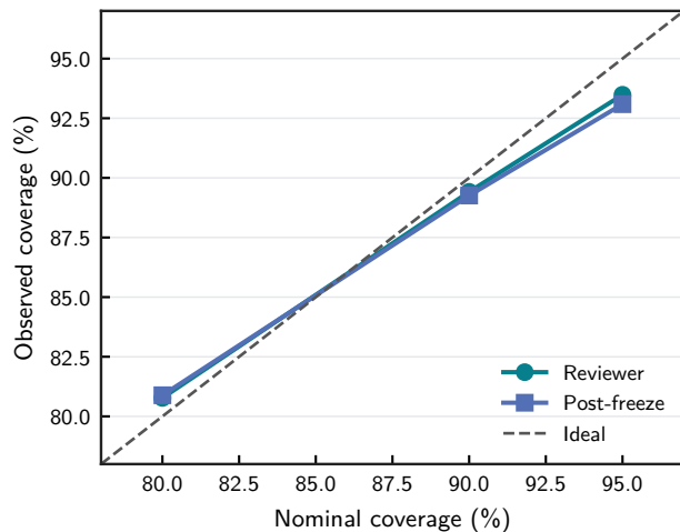
B Validation-only interval calibration
