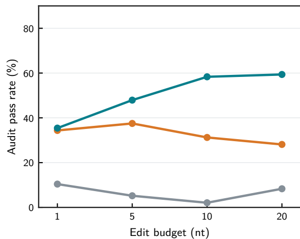
C HepG2
