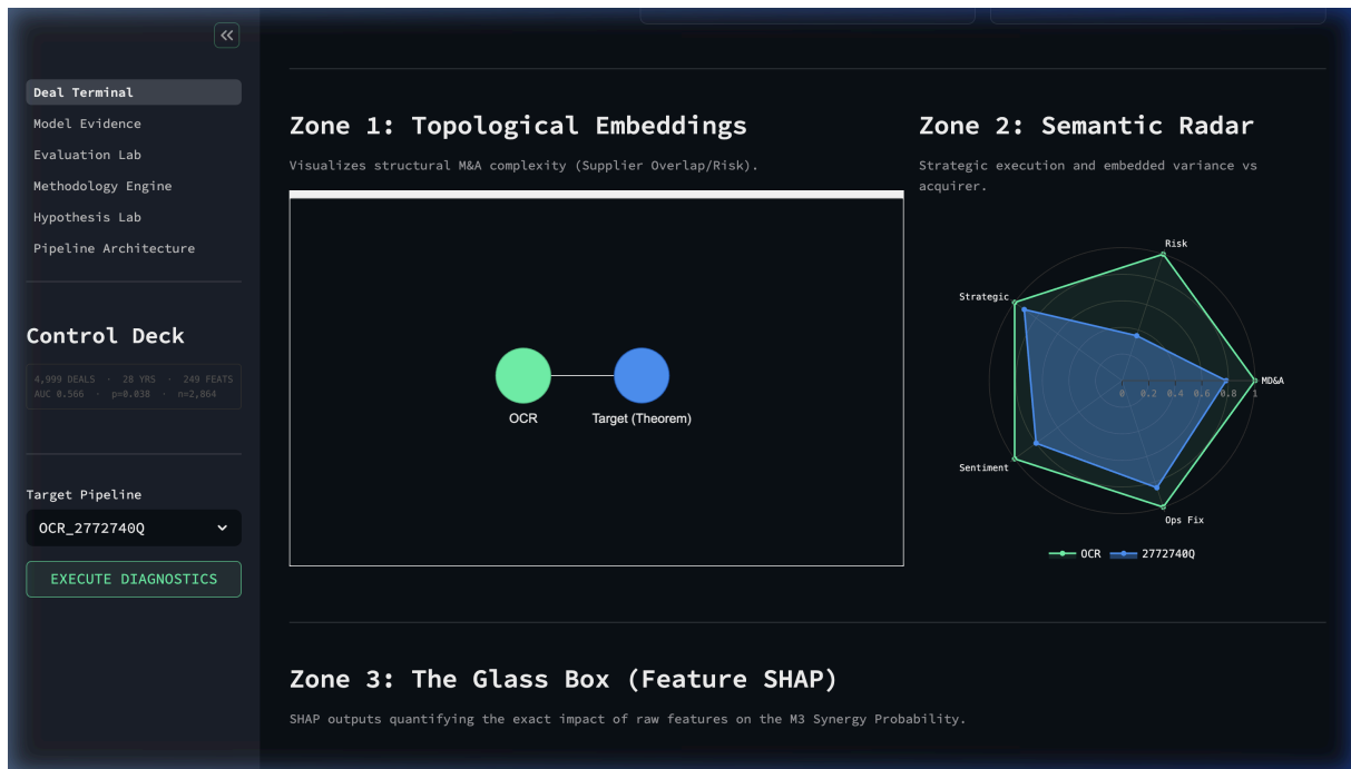
Figure 22: Zone 1 (Topological Embeddings) rendering the acquirer–target supply-chain sub-graph, and Zone 2 (Semantic Radar) plotting the pentagonal linguistic profile comparison.
