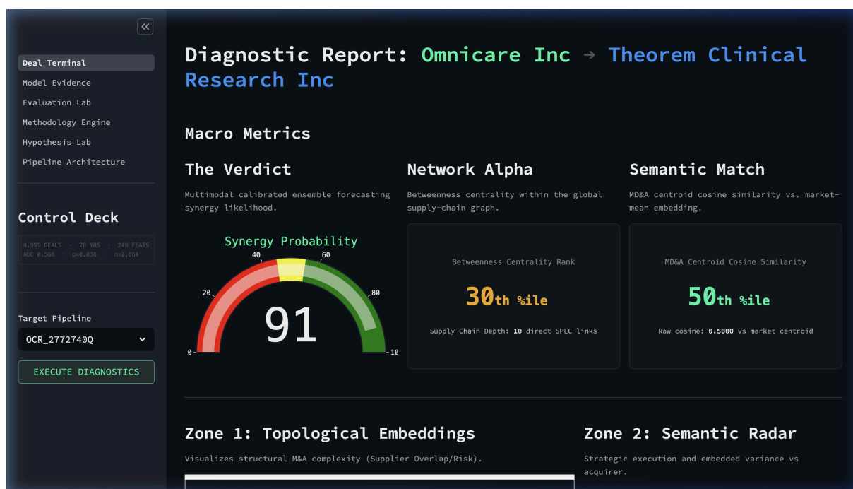
Figure 21: The diagnostic verdict showing a 91% synergy probability calibrated via the M3 ensemble, alongside betweenness centrality rank (30th percentile) and MD&A semantic match.
