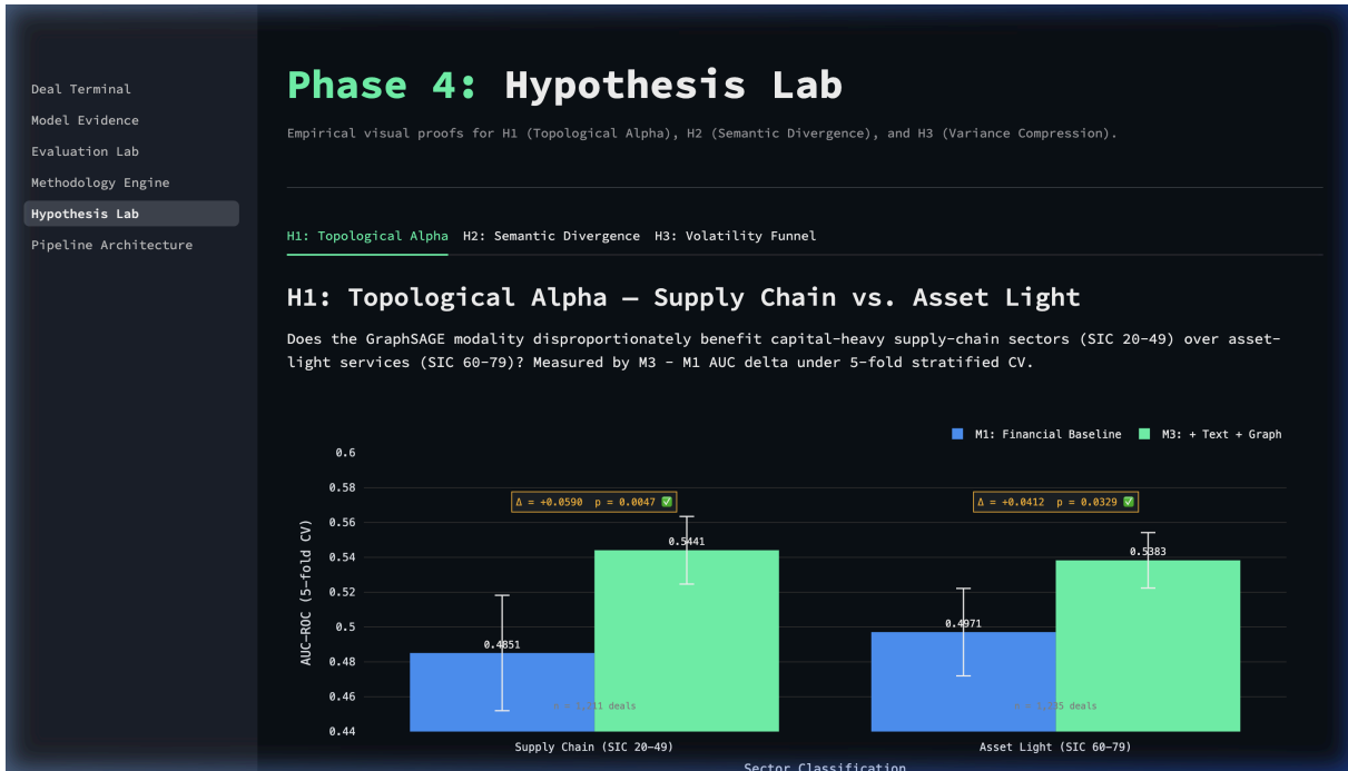
Figure 26: The Hypothesis Lab, showcasing the sector-wise AUC lift used to validate Hypothesis 1 (Topological Alpha) with \pm 1\sigma error bars.
