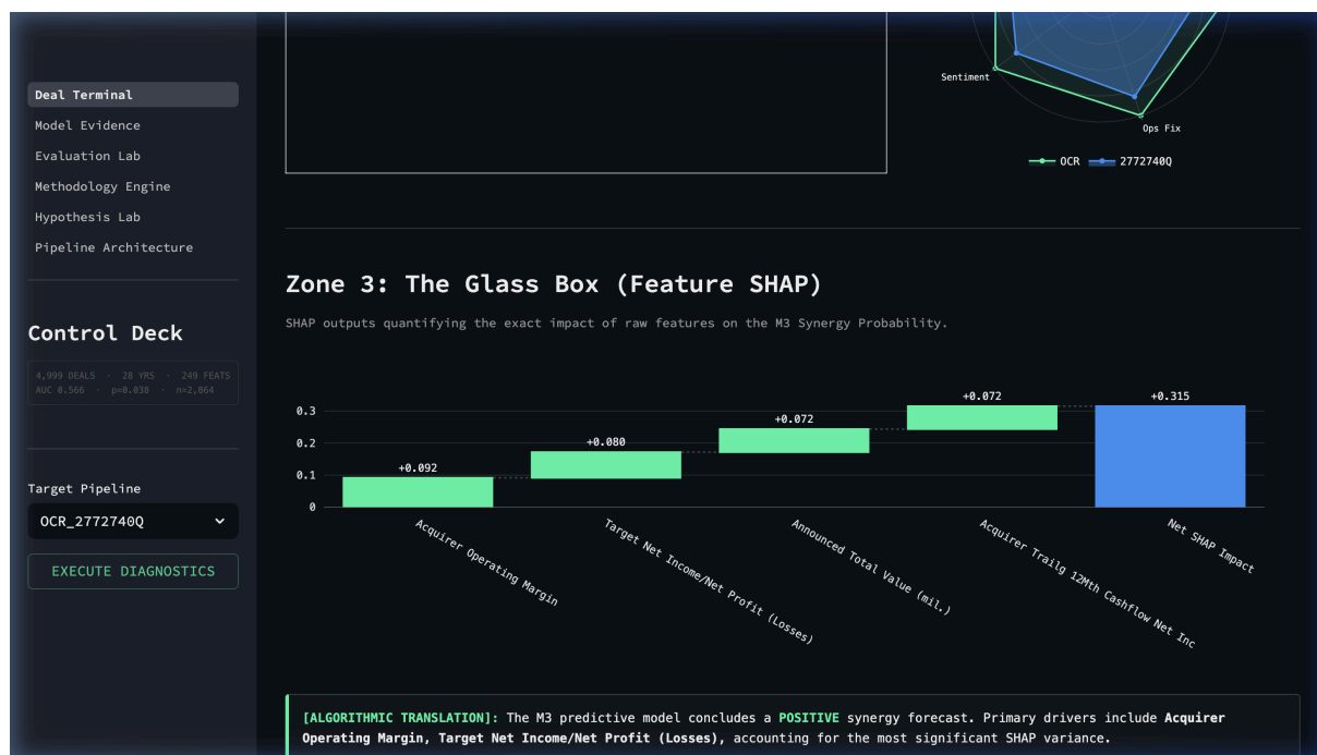
Figure 22: Zone 3: SHAP waterfall decomposition of the synergy probability, with the Algorithmic Translation summary below.
