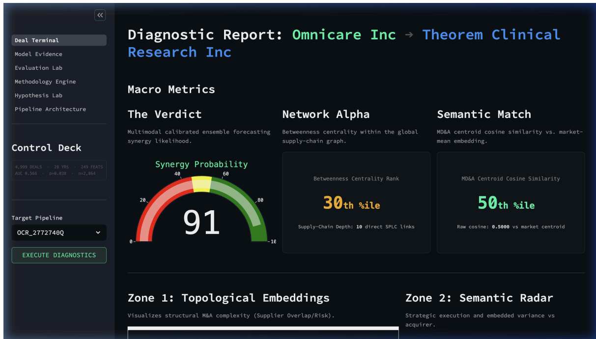
Figure 20: The diagnostic verdict showing a 91% synergy probability calibrated via the M3 ensemble, alongside betweenness centrality rank (30th percentile) and MD&A semantic match.
