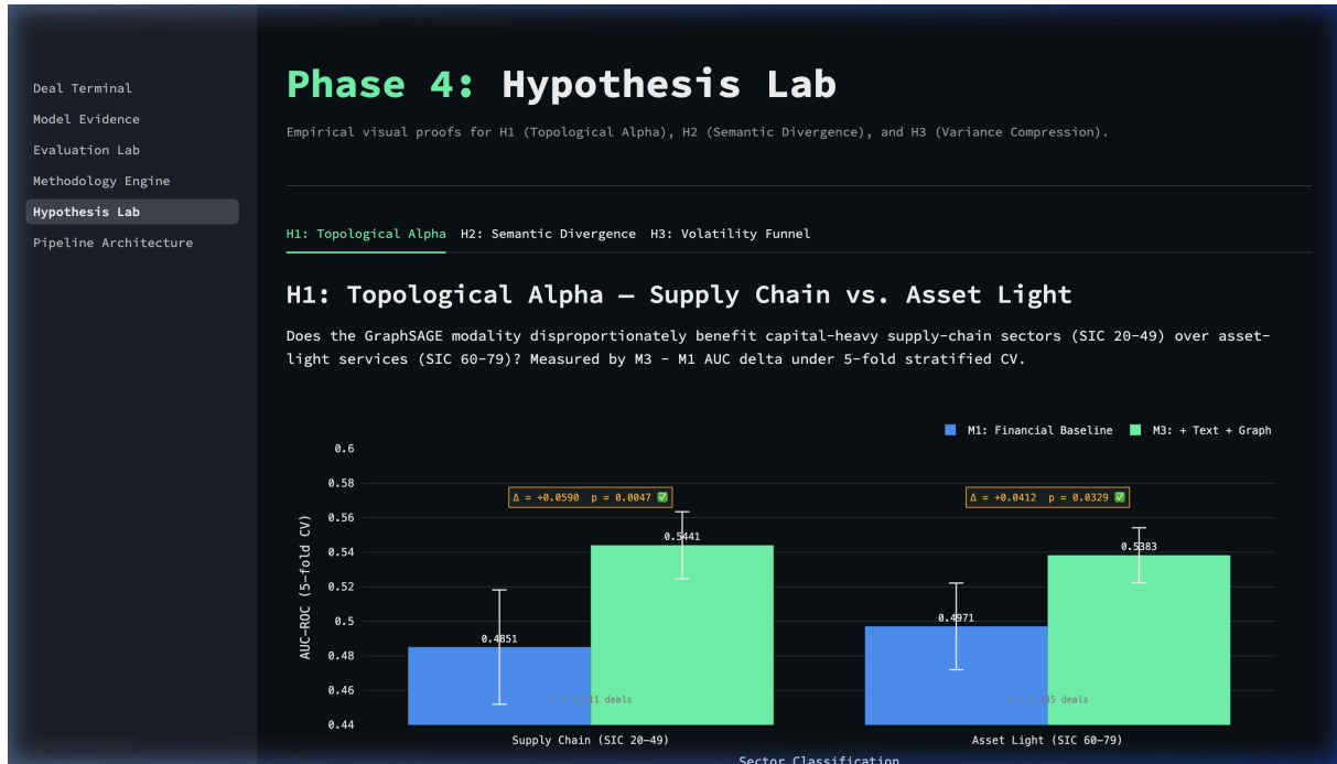
Figure 25: The Hypothesis Lab, showcasing the sector-wise AUC lift used to validate Hypothesis 1 (Topological Alpha) with \pm 1\sigma error bars.
