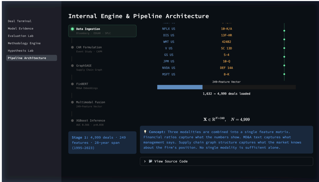
Figure 26: The Pipeline Architecture interface, documenting the internal tensor flow and the 249-dimensional multimodal feature concatenation logic. 3
