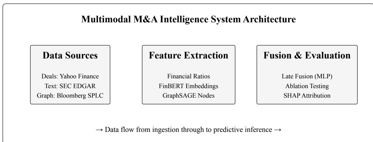
Figure 1: System architecture pipeline showing the integration of Yahoo Finance deal data, SEC textual data, and Bloomberg topological data.
