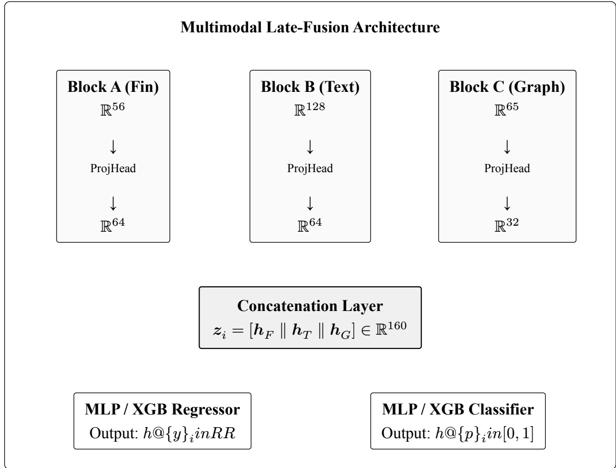
Figure 5: Multimodal late-fusion architecture. The raw concatenated features (249-dim) are projected into a 160-dimensional joint representation z_i before entering the prediction heads.
