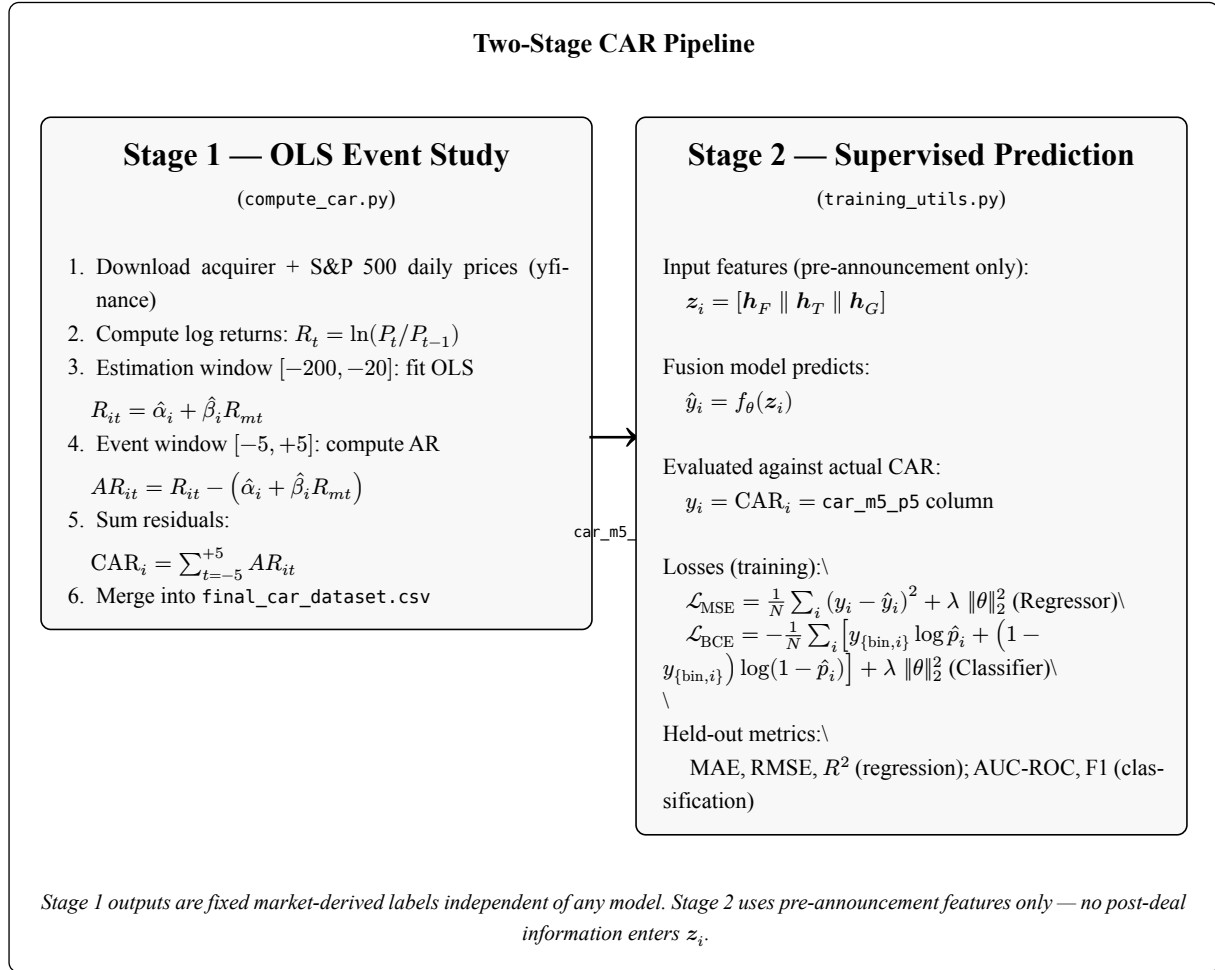
Listing 2: The two-stage CAR pipeline: Stage 1 computes actual CAR via OLS event study; Stage 2 trains and evaluates the fusion model against those labels.
