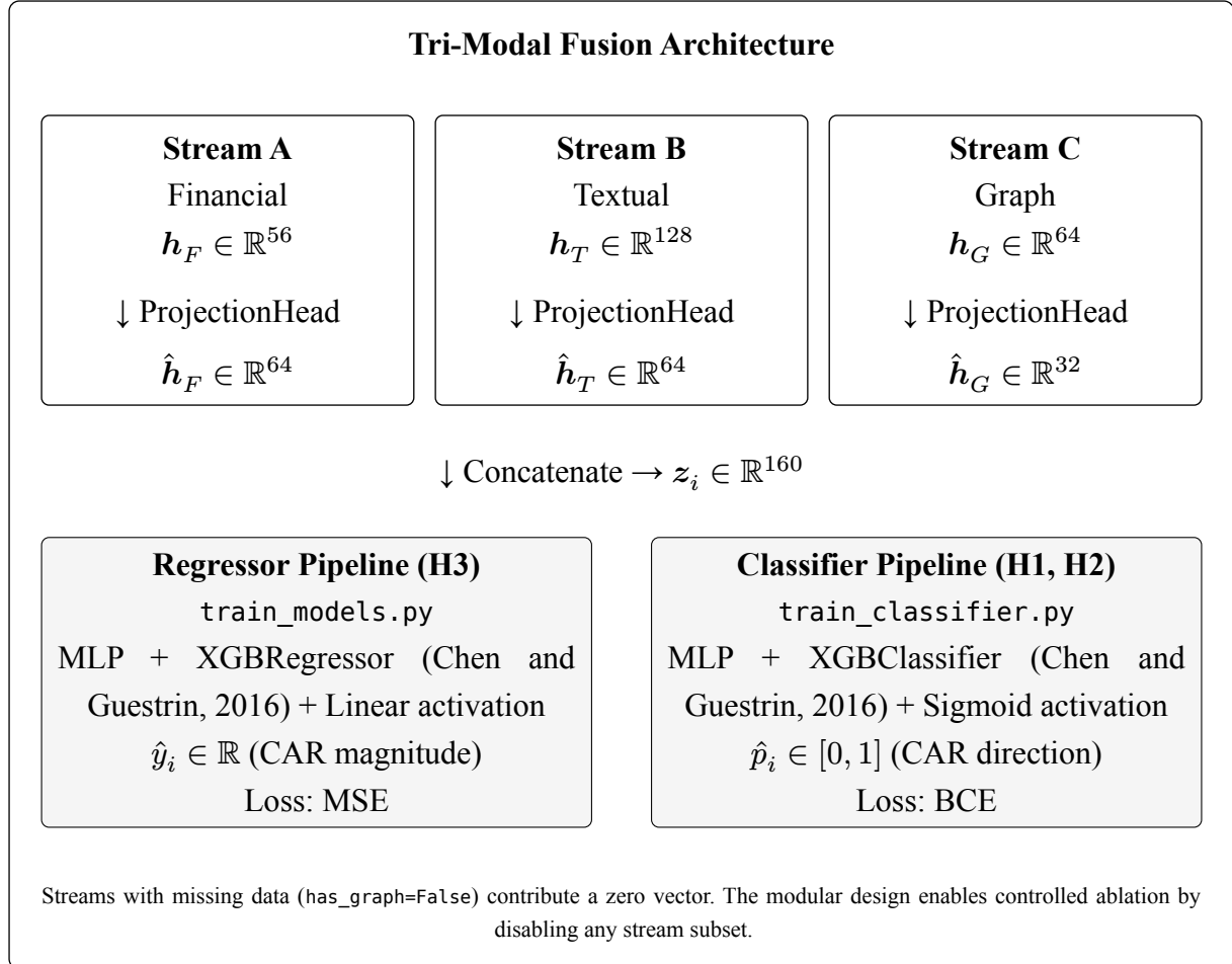
Listing 1: Tri-modal late-fusion architecture (src/models/fusion.py).
