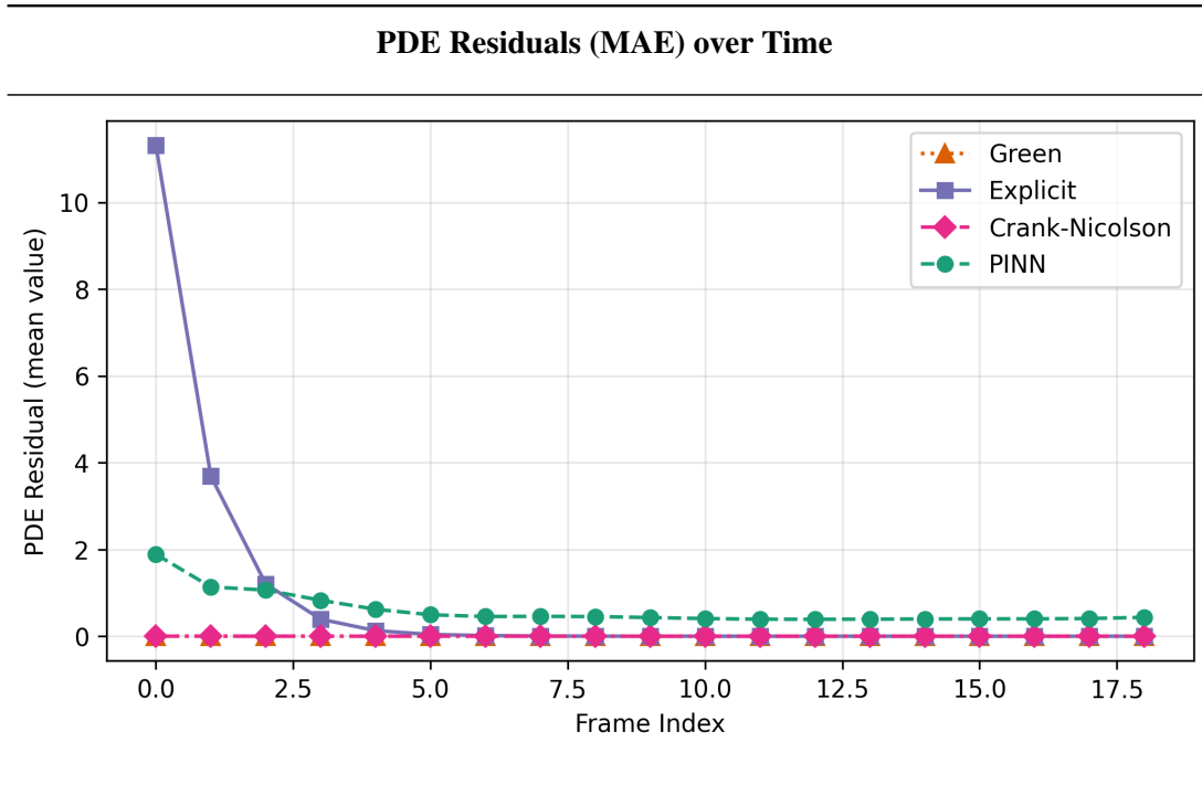
Figure 4: PDE Residuals (MAE) over Time.
