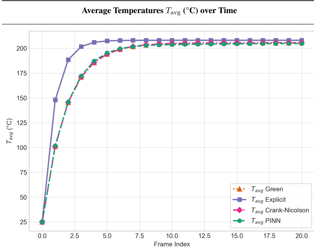
Figure 3: Average Temperatures over Time.
