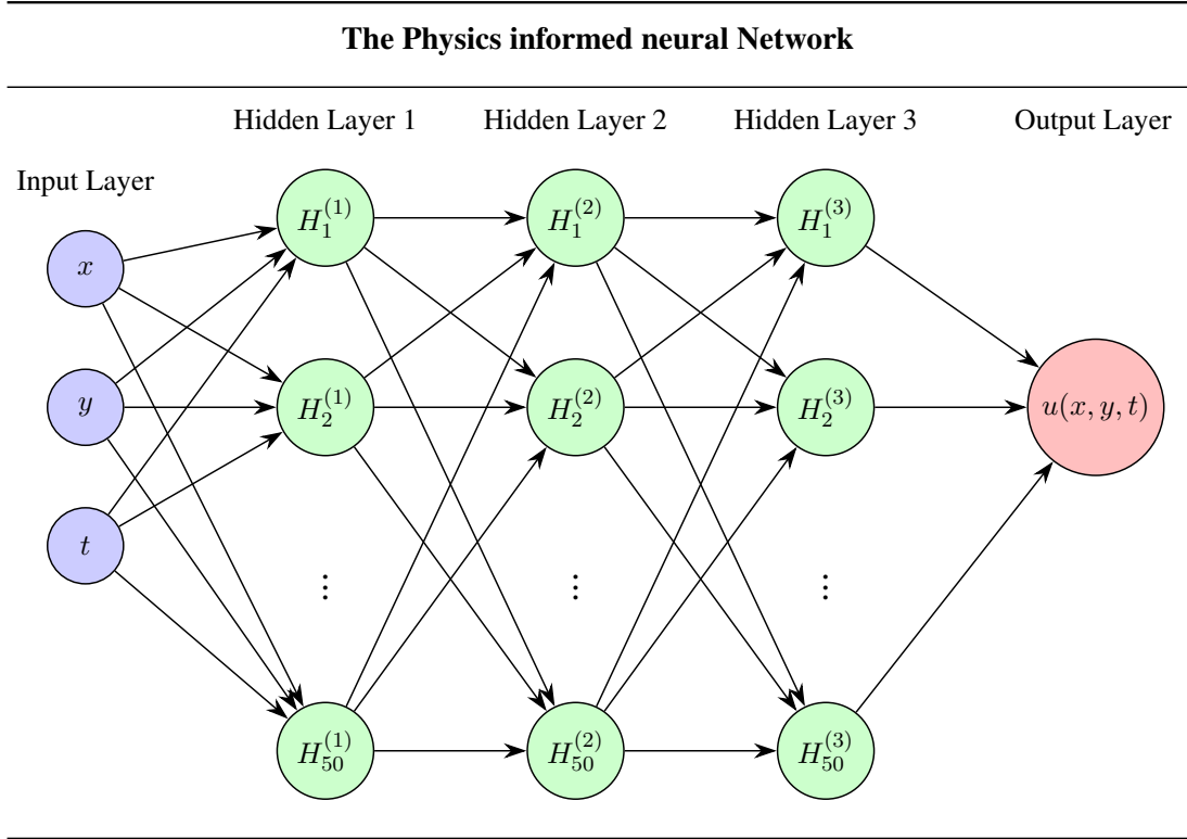
Figure 2: The Physics informed neural Network (PINN)
